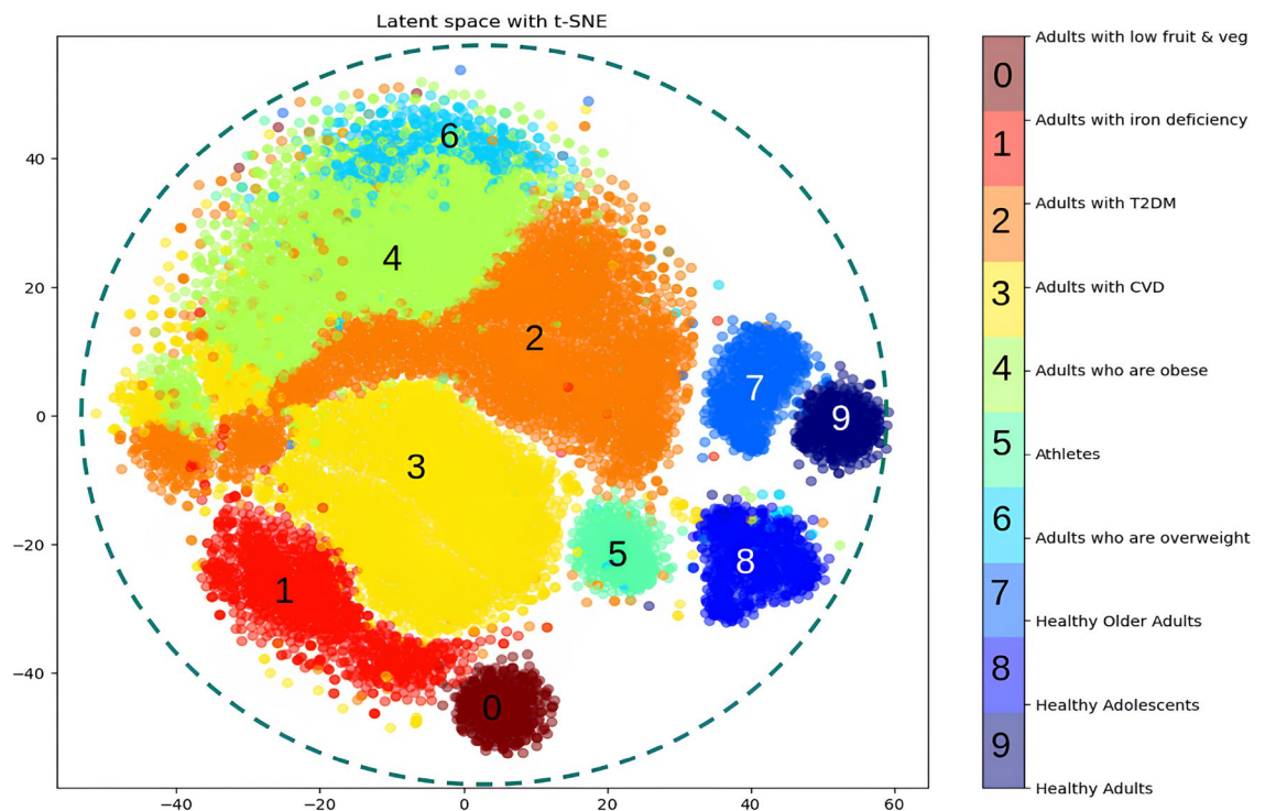
Figure 5. Visualization of the latent space for 3000 user profiles.
