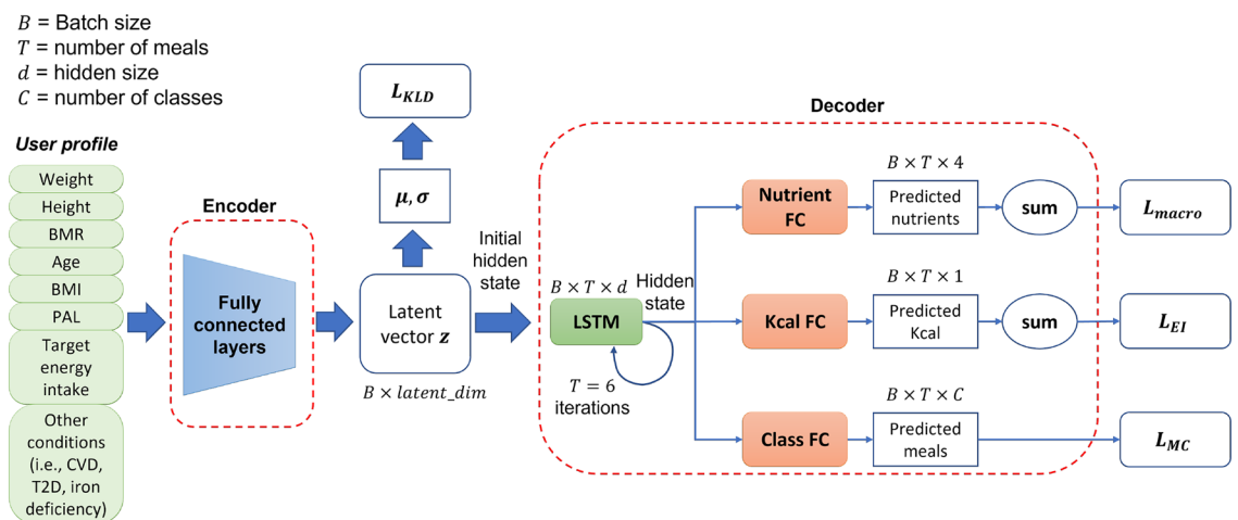
Figure 2. Internal architecture of the variational autoencoder.
